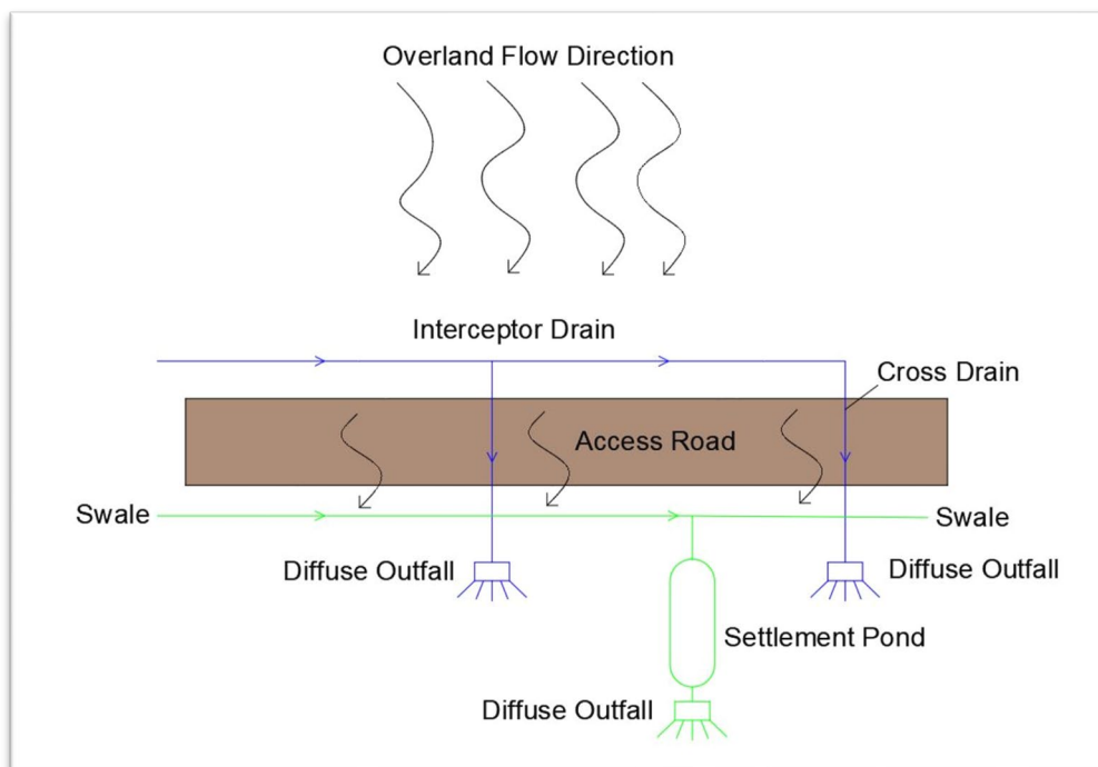
Figure 2-4: Drainage Diagram
