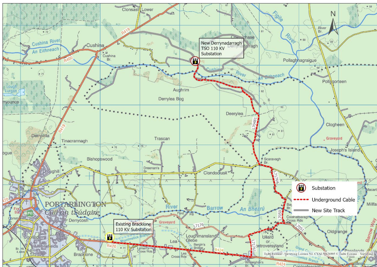
Figure 2-1: Grid Connection Route
